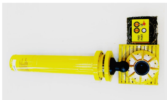
Bowl/ball piston rod end and inconell clad piston rod
